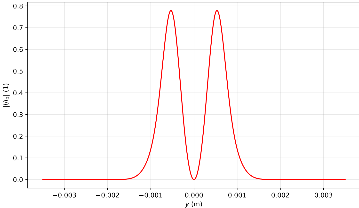
Intensity profile I(x=0, y, z=0.637)/I_0 , P_{in}=2.0P_{cr} , artificial time
